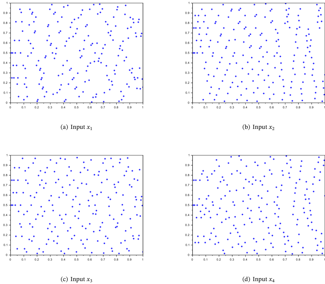
Figure 3: Distribution of Sobol sequences for each model input for n = 200 .
