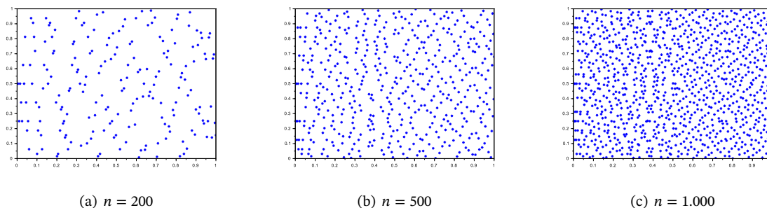
Figure 6: Distribution of Sobol sequences for input x_1 ad n = 200, n = 500 e n = 1.000 .
