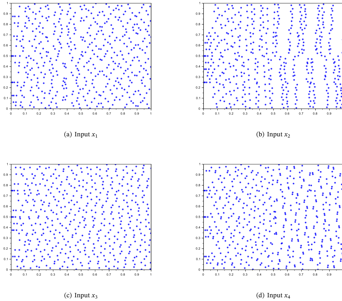
Figure 4: Distribution of Sobol sequences for each model input for n = 500 .
