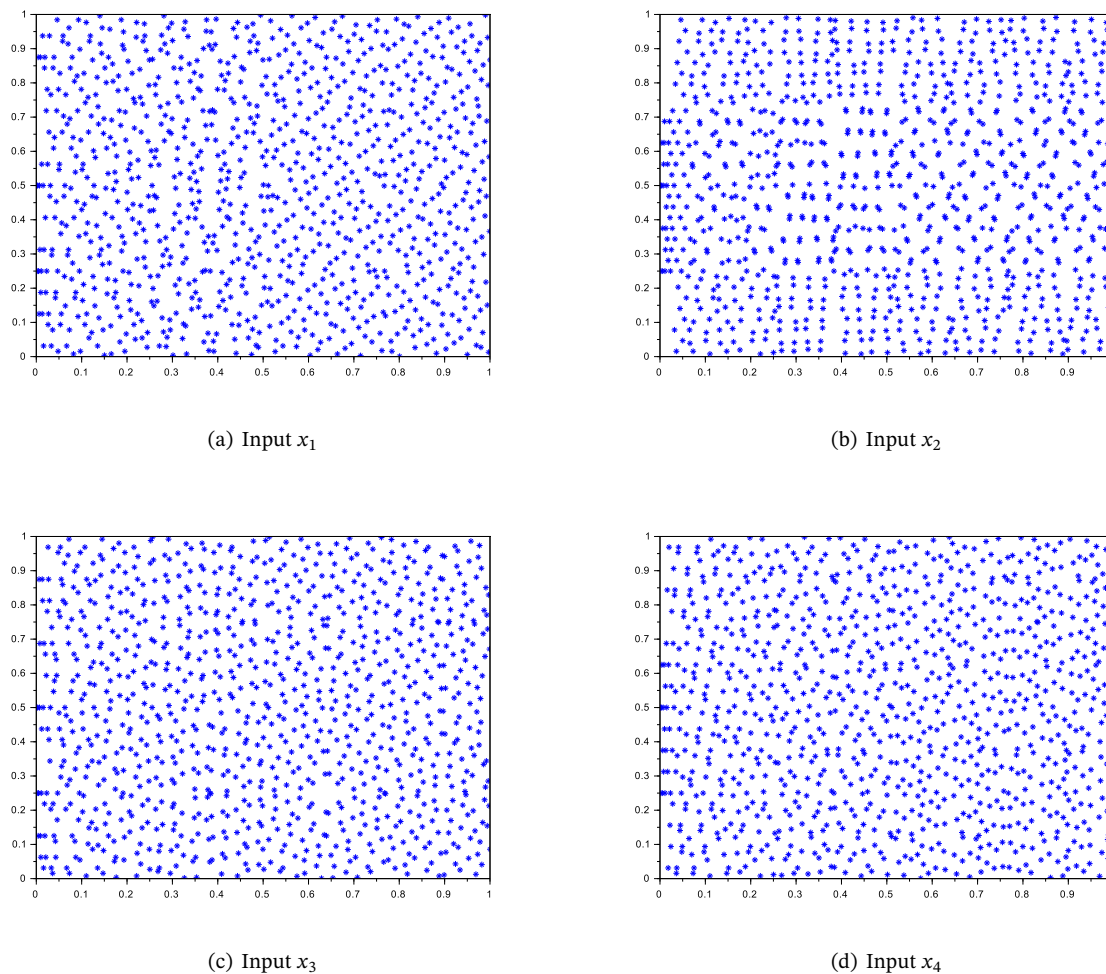
Figure 5: Distribution of Sobol sequences for each model input for n = 1000 .
